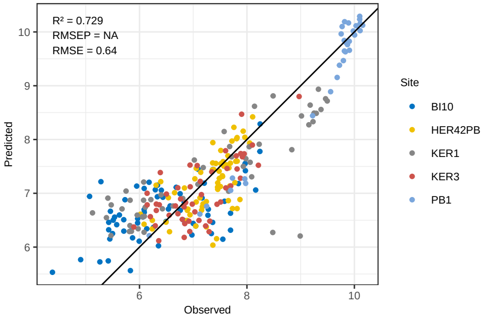
Ti WLS_weighted – Predicted vs Observed
