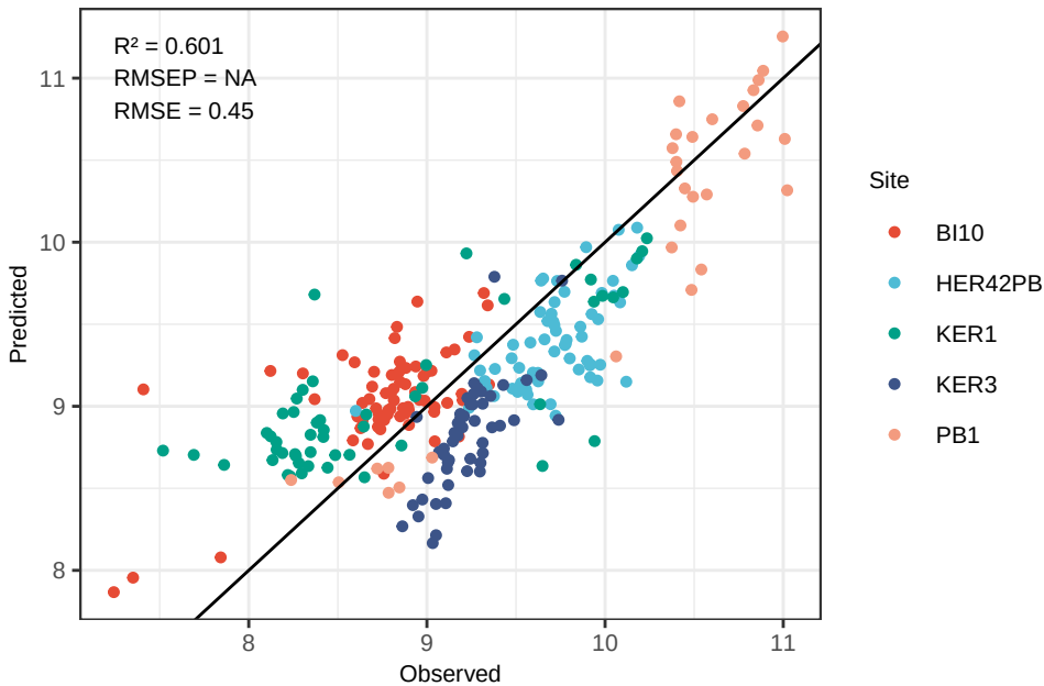
Ca OLS_weighted – Predicted vs Observed
