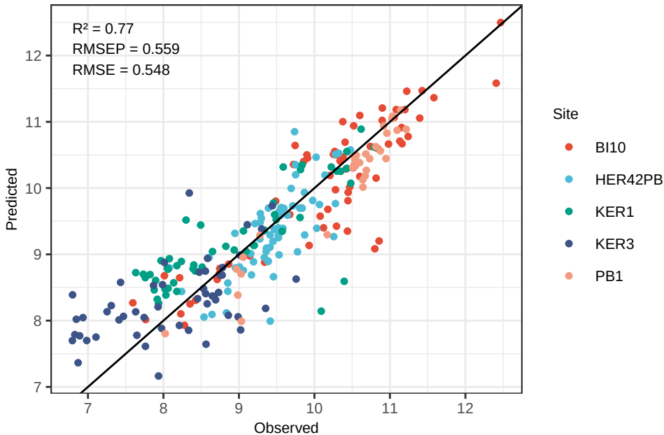
Fe PLS_LOO – Predicted vs Observed
