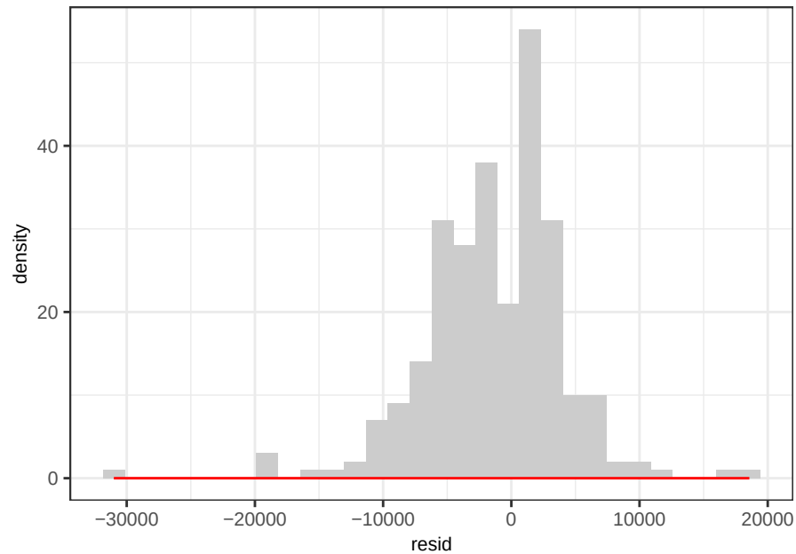
Ca OLS_weighted - ACE Residuals
