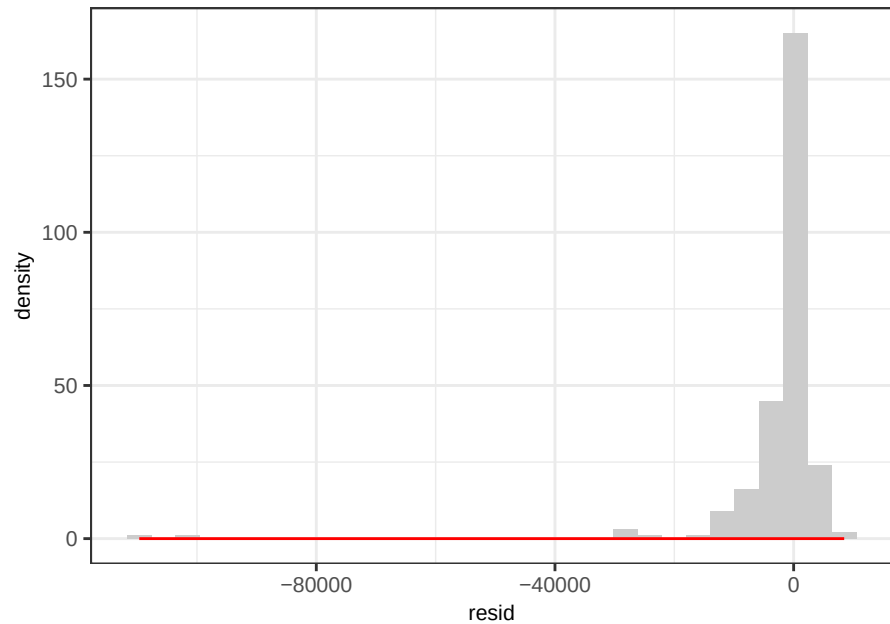
Fe RF - ACE Residuals
