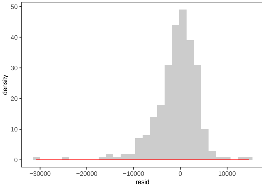
Ca Bayes - ACE Residuals
