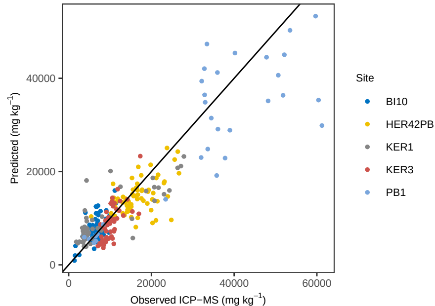
Ca PLS_kfold – Predicted vs Observed
