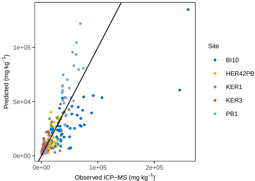
Fe OLS_weighted – Predicted vs Observed
