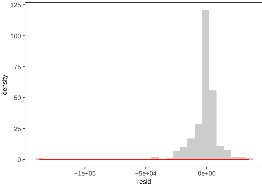
Fe PLS_kfold - ACE Residuals
