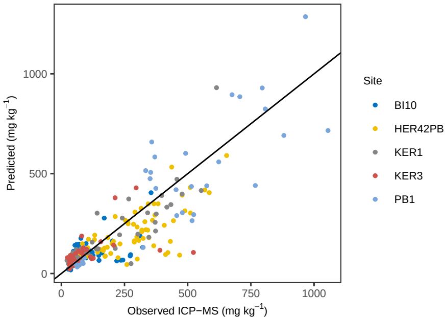
Mn Bayes – Predicted vs Observed
