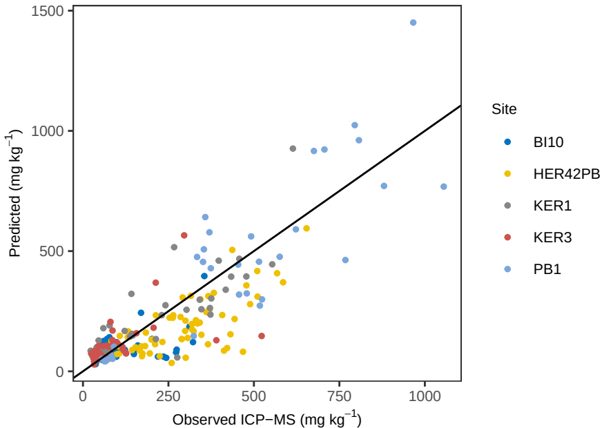
Mn OLS – Predicted vs Observed
