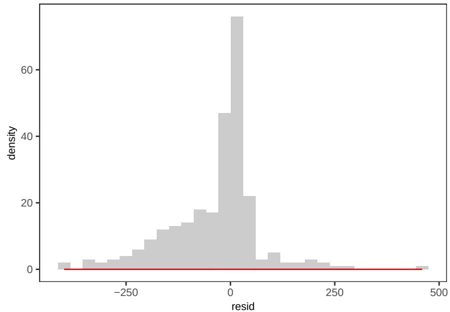
Mn OLS_weighted - ACE Residuals
