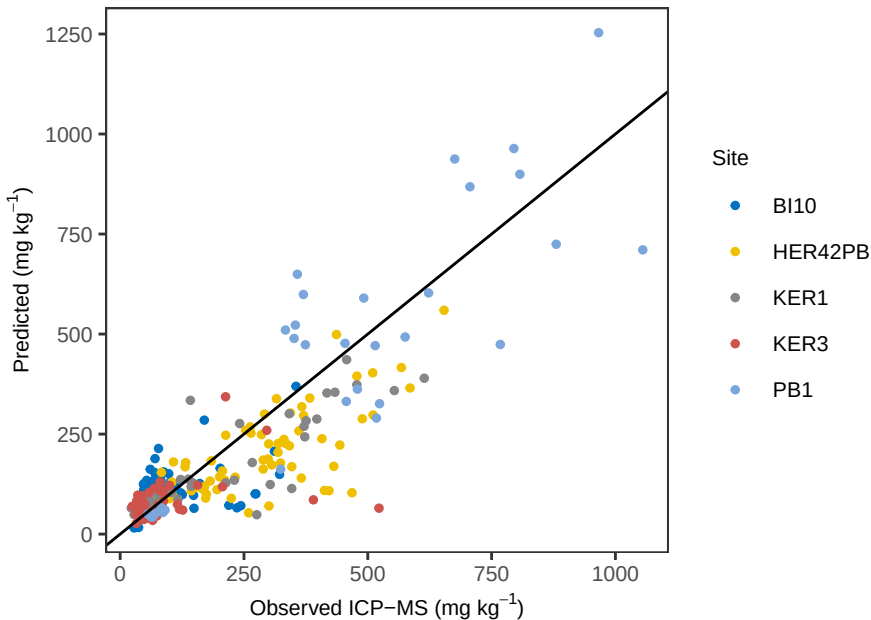
Mn PLS_LOO – Predicted vs Observed
