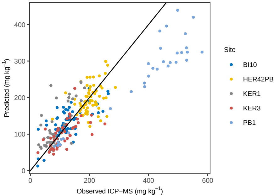
Sr PLS_LOO - Predicted vs Observed
