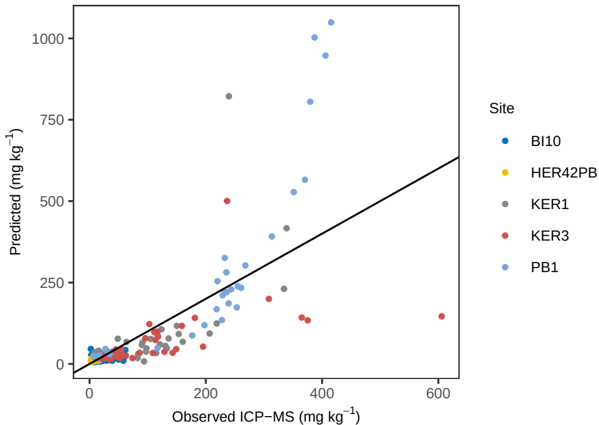
Zr PLS_kfold - Predicted vs Observed
