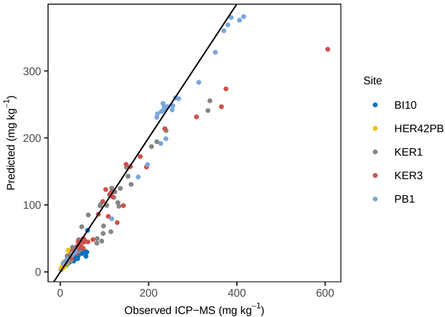
Zr RF – Predicted vs Observed
