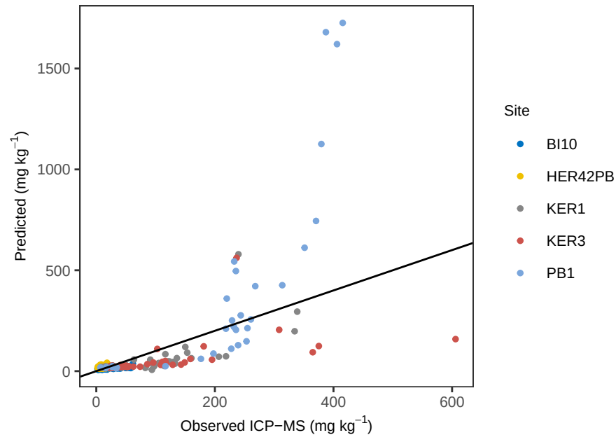
Zr WLS – Predicted vs Observed
