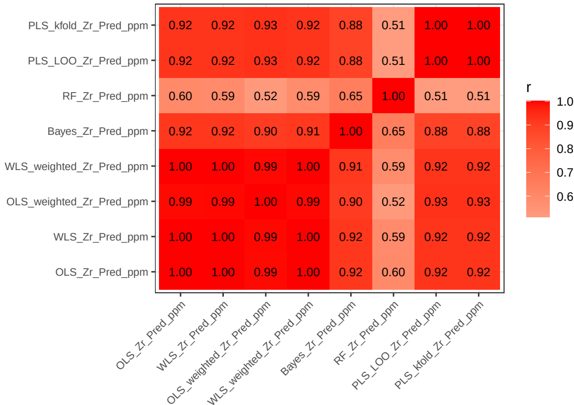
Model prediction correlation – Zr
