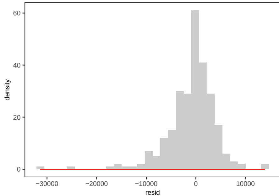
Ca PLS_LOO - ACE Residuals
