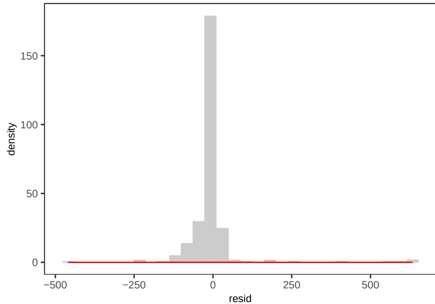
Zr PLS_LOO - ACE Residuals
