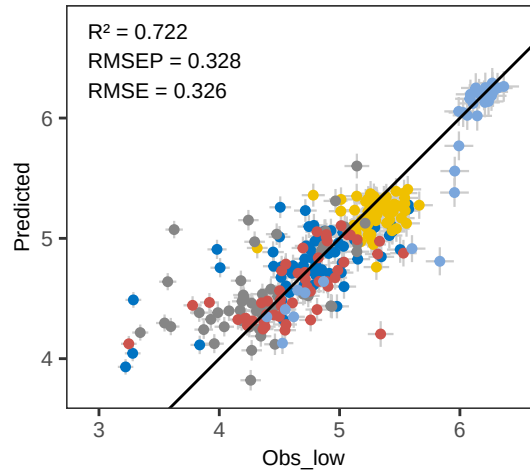
Sr PLS_LOO – Predicted vs Observed
