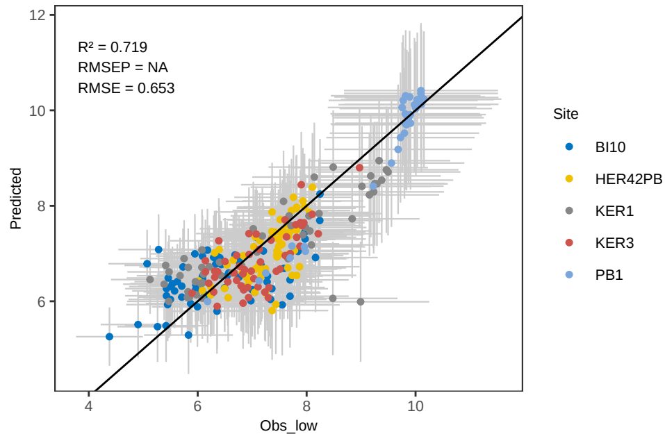
Ti OLS_weighted - Predicted vs Observed
