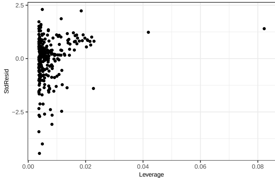
Sr OLS - Leverage
