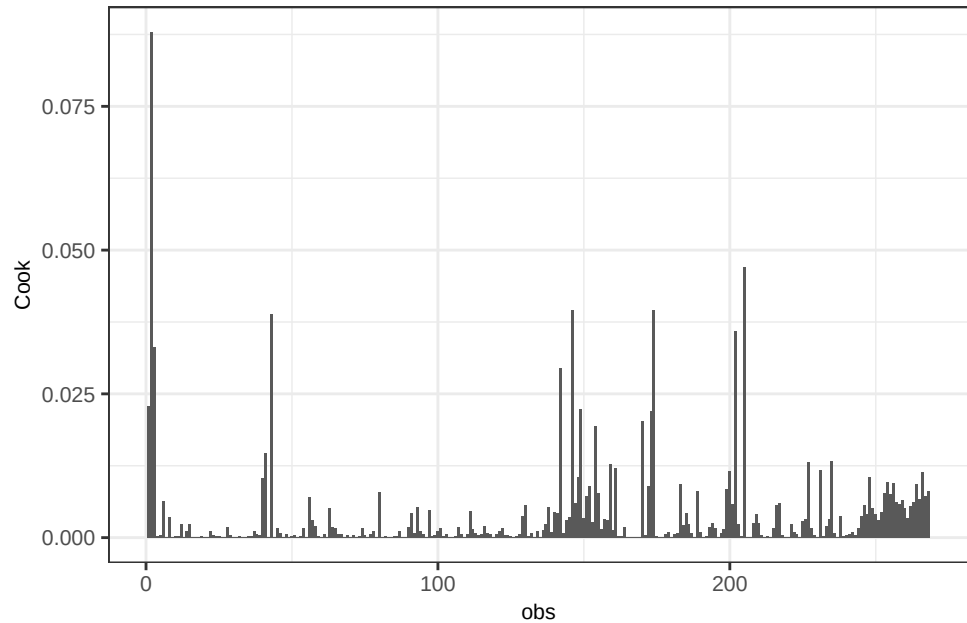
Sr OLS – Cook's Distance
