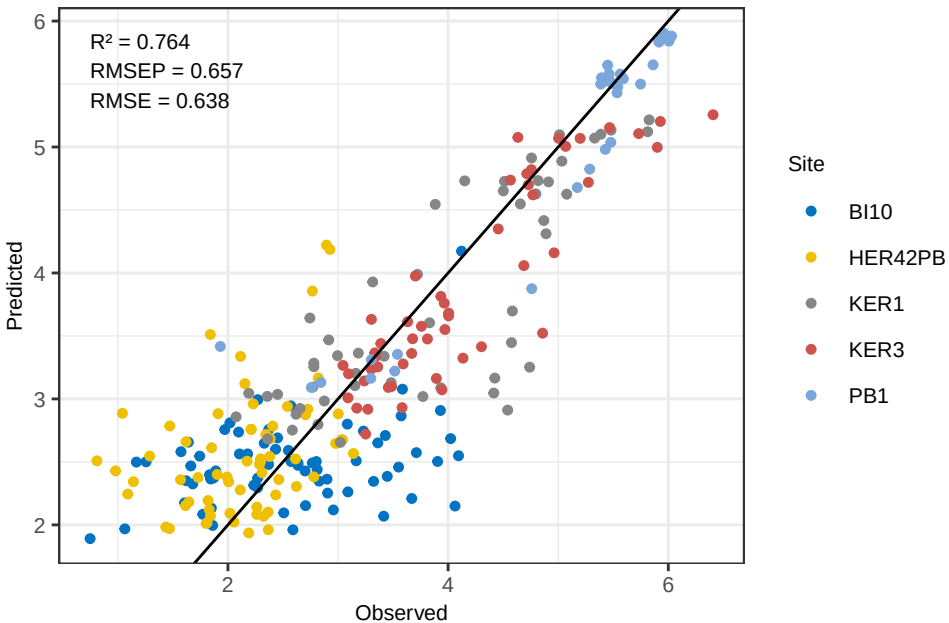
Zr RF – Predicted vs Observed
