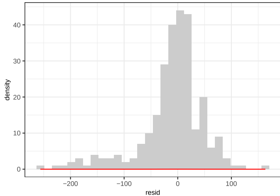
Sr PLS_LOO - ACE Residuals
