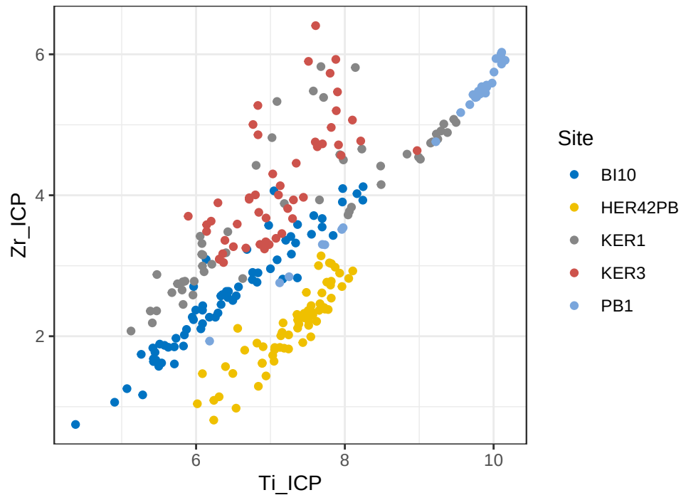
ICP relationship: Ti_ICP vs Zr_ICP
