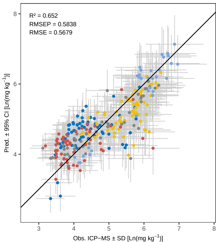
Mn PLS_LOO – Predicted vs Observed
