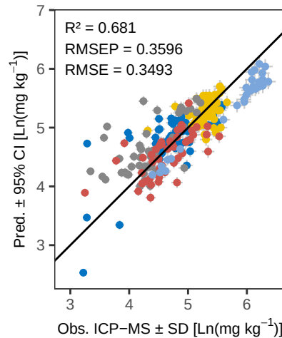
Sr PLS_LOO – Predicted vs Observed
