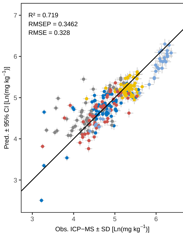
Sr Bayes – Predicted vs Observed
