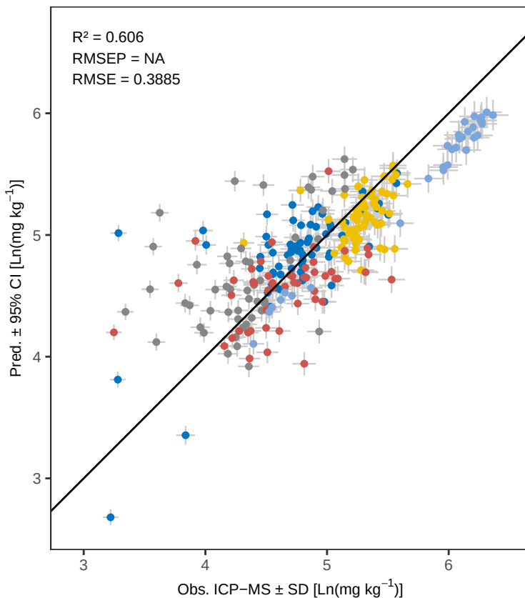
Sr WLS – Predicted vs Observed
