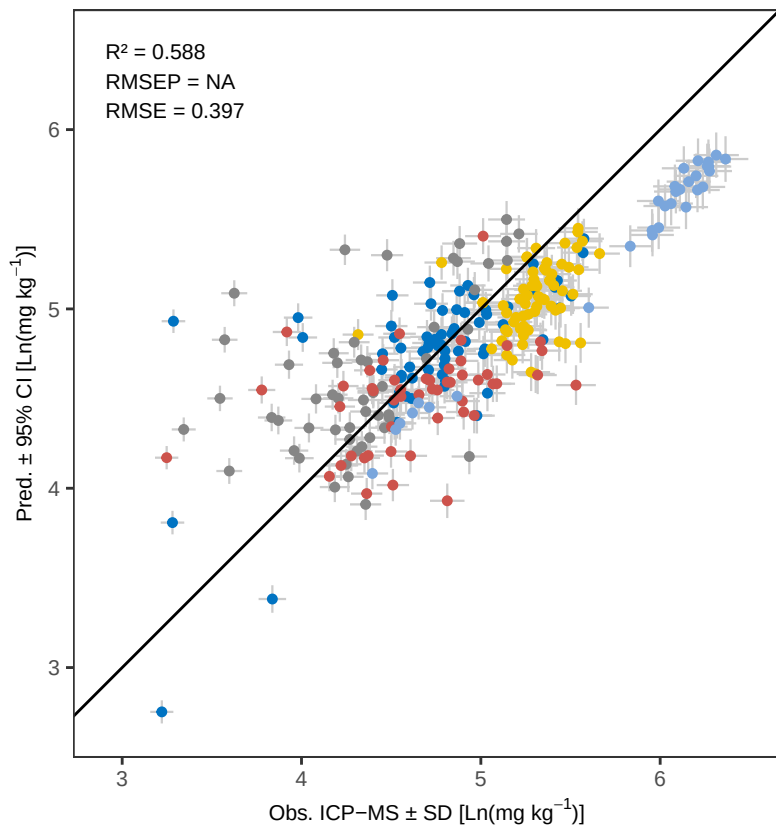
Sr OLS_weighted – Predicted vs Observed
