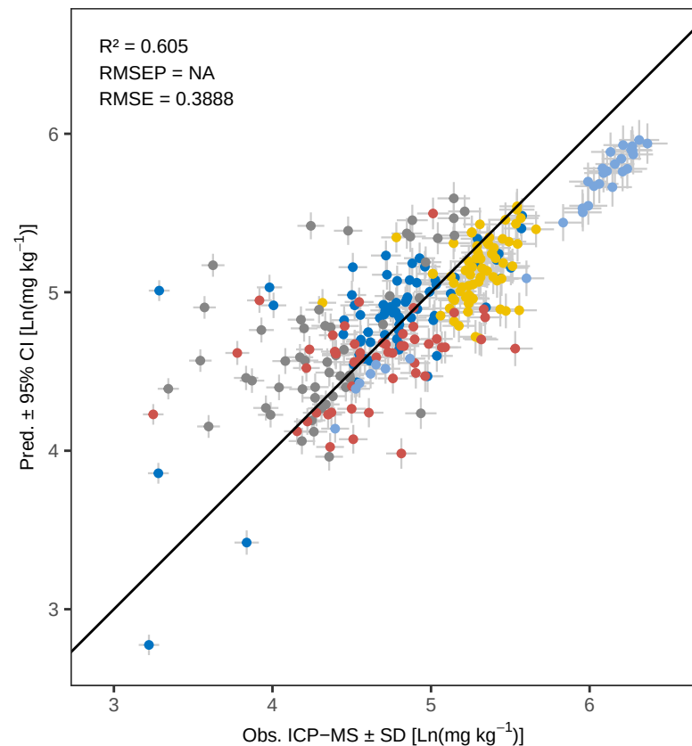
Sr WLS_weighted – Predicted vs Observed
