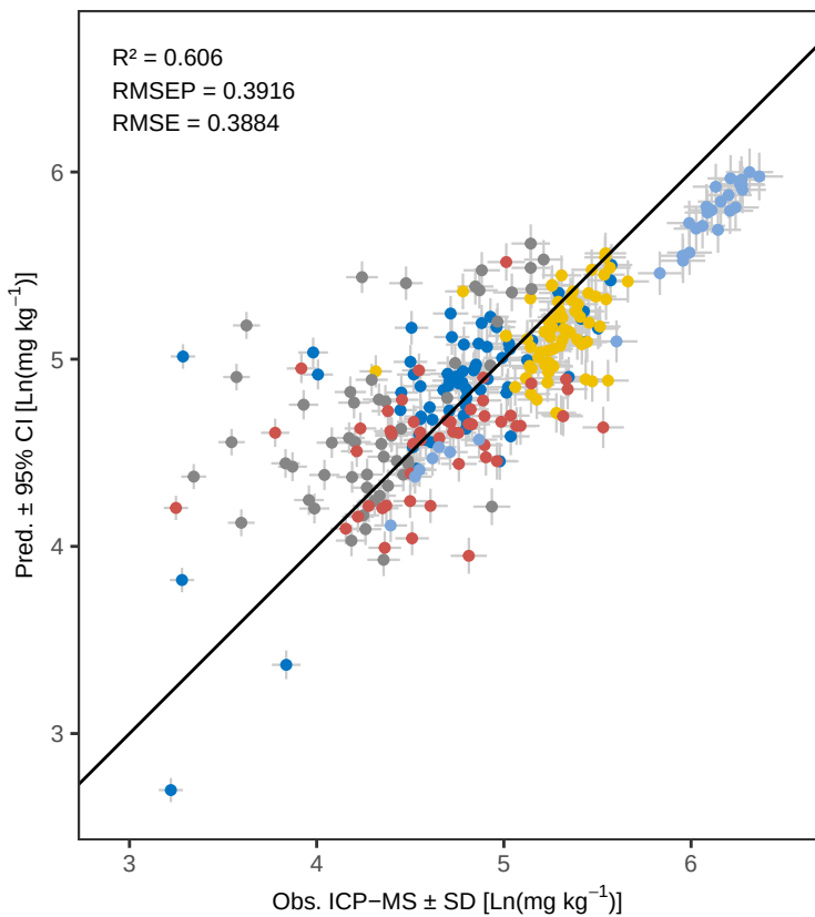
Sr OLS – Predicted vs Observed
