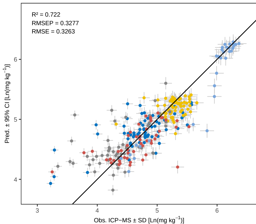
Sr RF – Predicted vs Observed
