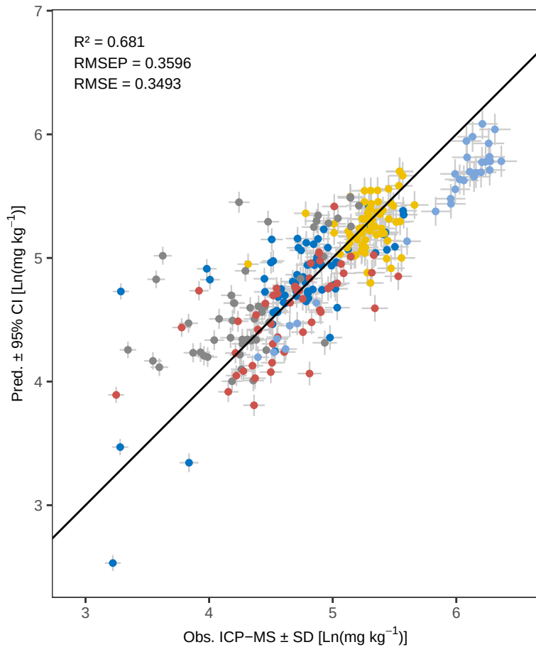
Sr PLS_LOO – Predicted vs Observed
