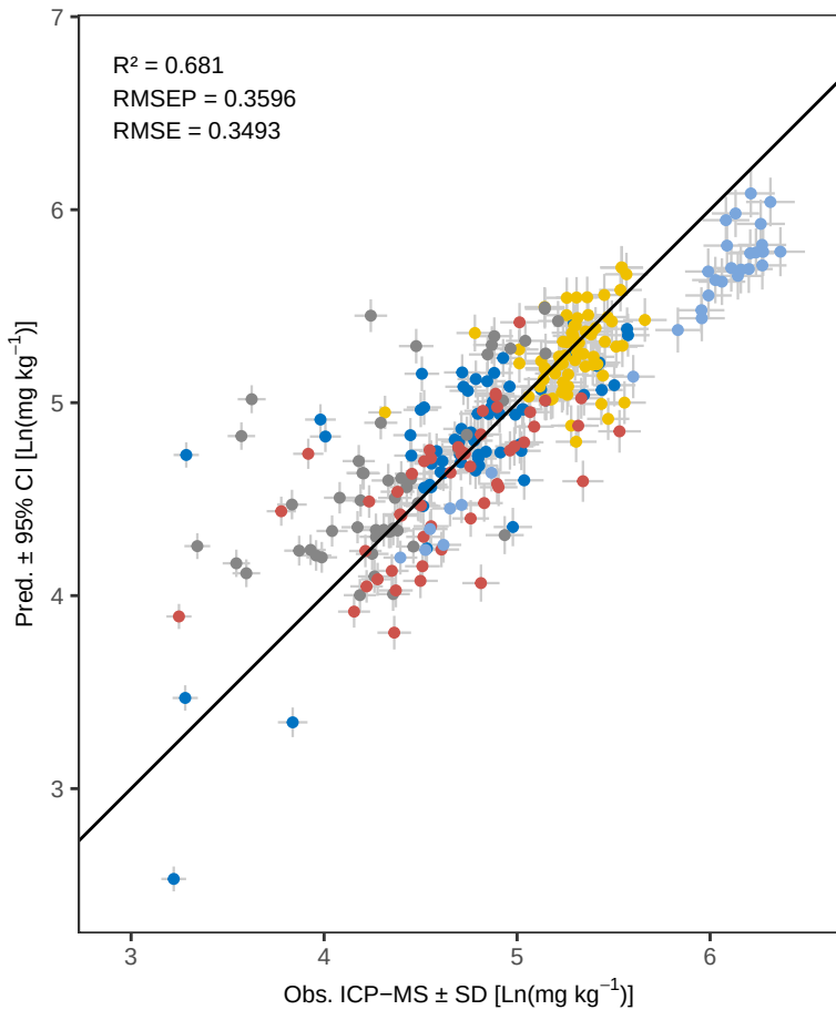
Sr PLS_kfold – Predicted vs Observed
