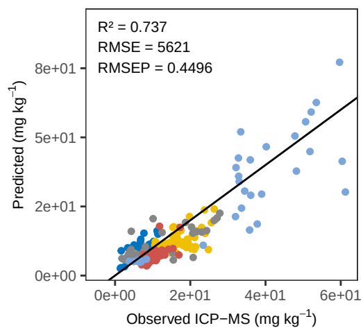
Ca WLS_weighted – ACE Predicted vs Observed
