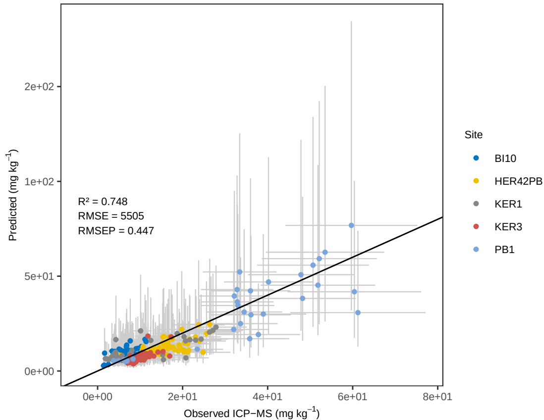
Ca OLS – ACE Predicted vs Observed (with errors)
