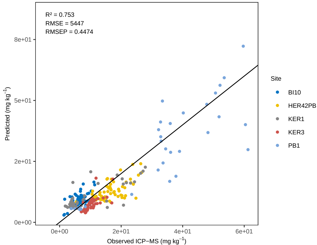
Ca WLS_weighted – ACE Predicted vs Observed
