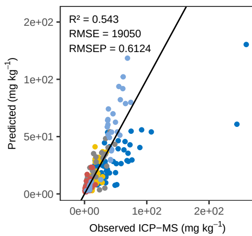
Fe WLS – ACE Predicted vs Observed
