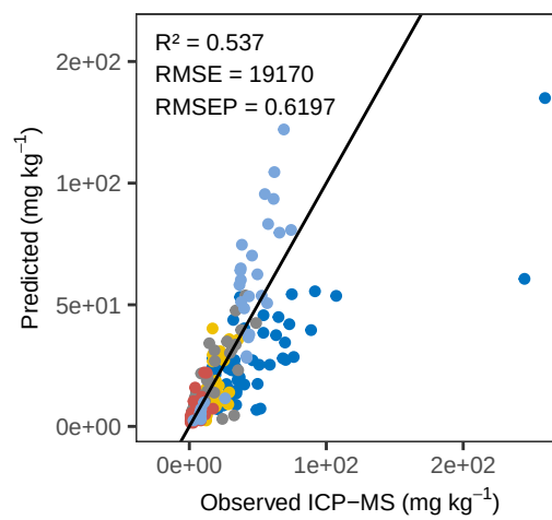
Fe WLS_weighted – ACE Predicted vs Observed
