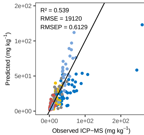
Fe RF – ACE Predicted vs Observed
