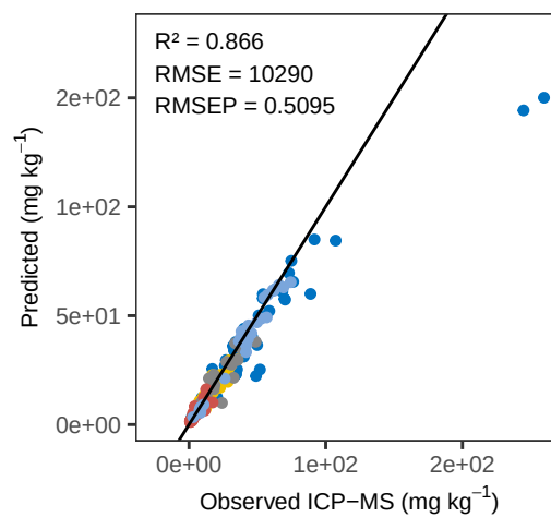
Fe PLS_LOO – ACE Predicted vs Observed
