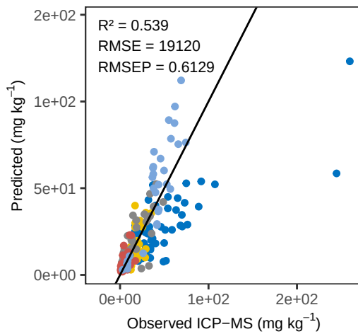
Fe Bayes – ACE Predicted vs Observed
