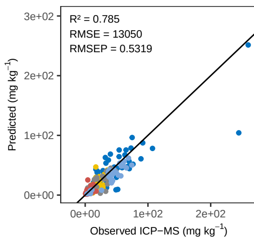
Fe PLS_kfold – ACE Predicted vs Observed
