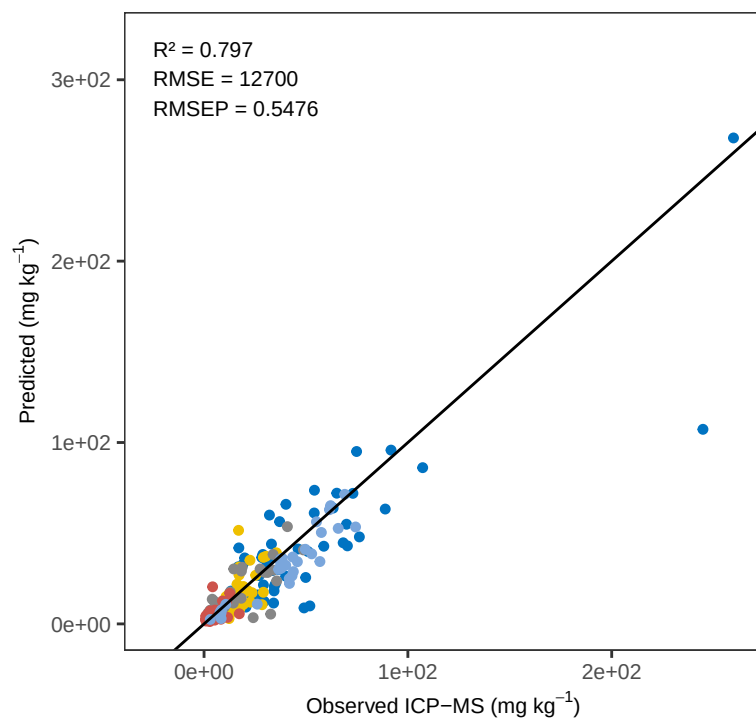
Fe PLS_LOO – ACE Predicted vs Observed
