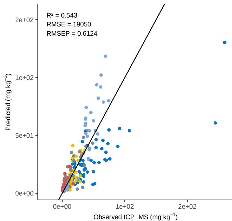
Fe OLS – ACE Predicted vs Observed
