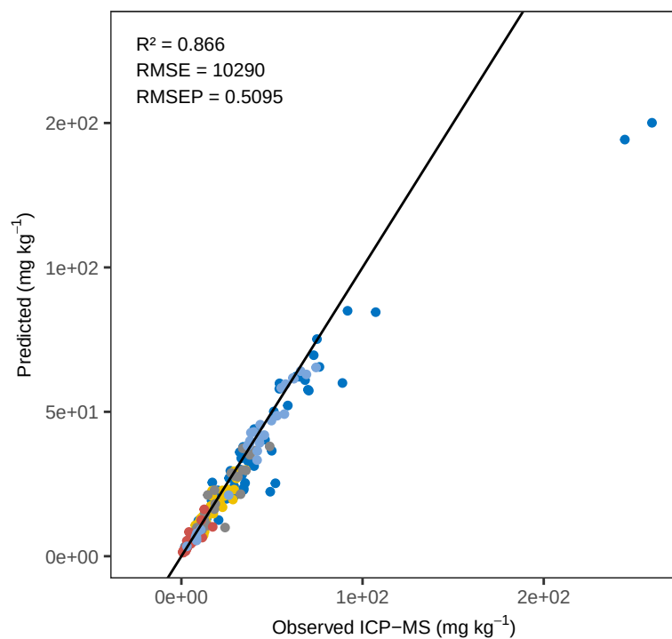
Fe RF – ACE Predicted vs Observed
