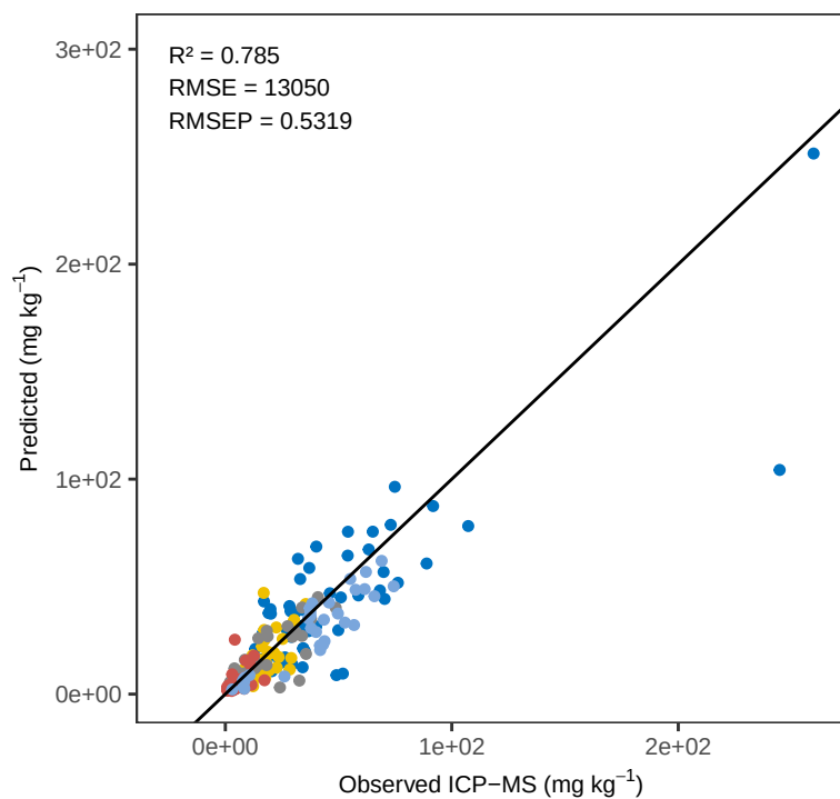
Fe Bayes – ACE Predicted vs Observed
