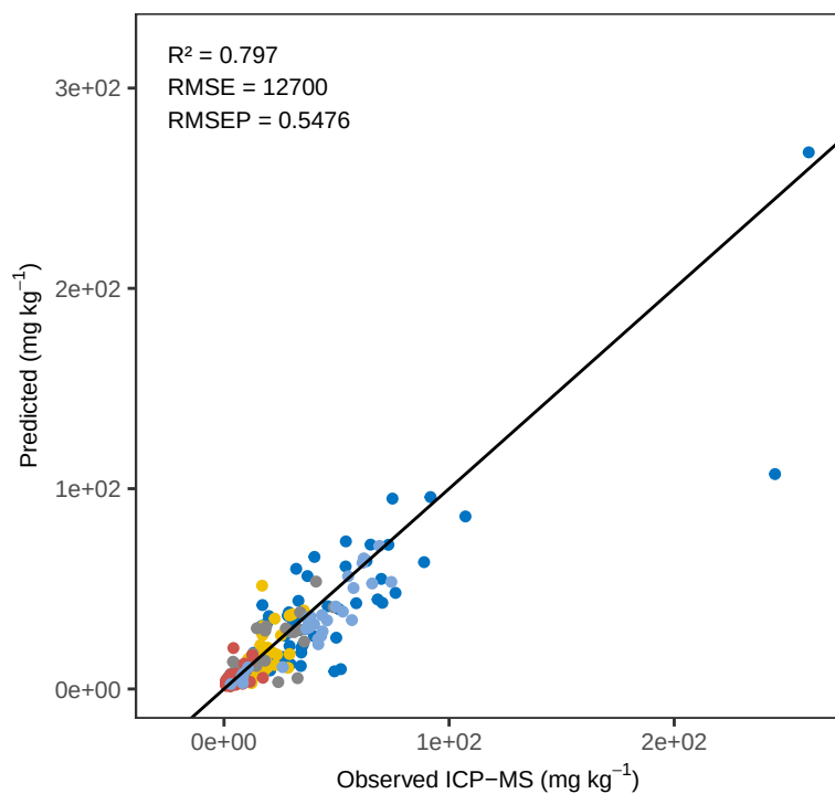
Fe PLS_kfold – ACE Predicted vs Observed
