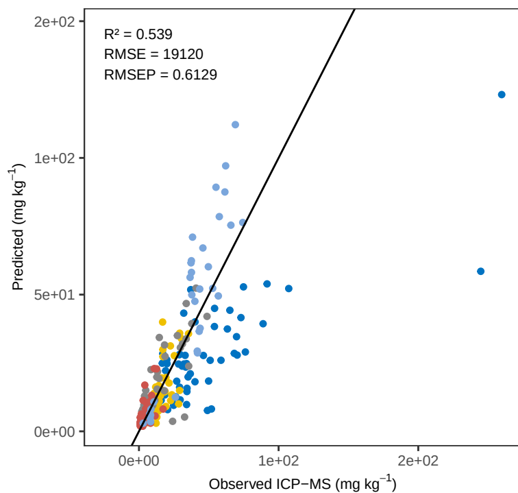
Fe WLS – ACE Predicted vs Observed
