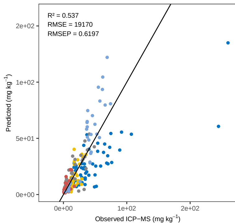
Fe OLS_weighted – ACE Predicted vs Observed
