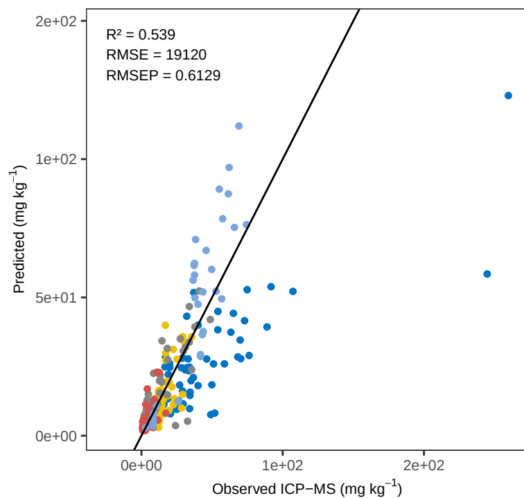
Fe WLS_weighted – ACE Predicted vs Observed
