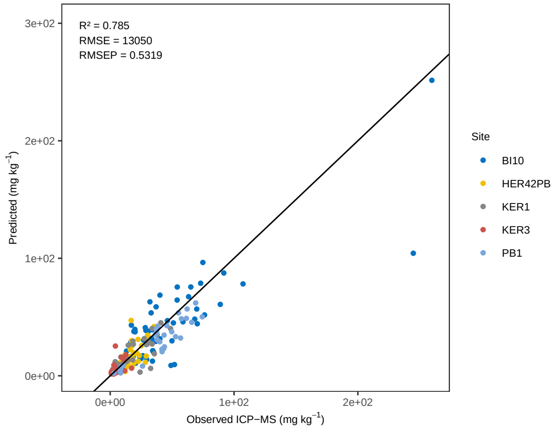
Fe Bayes – ACE Predicted vs Observed
