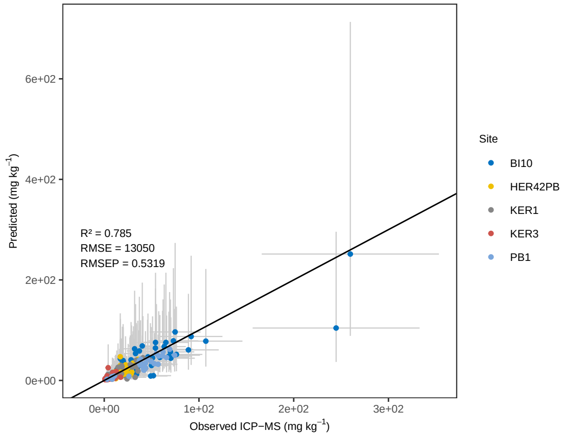
Fe Bayes – ACE Predicted vs Observed (with errors)
