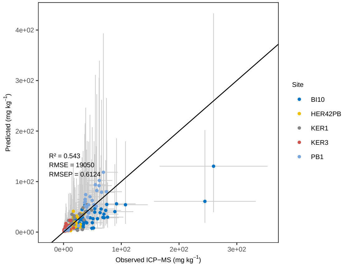
Fe OLS – ACE Predicted vs Observed (with errors)
