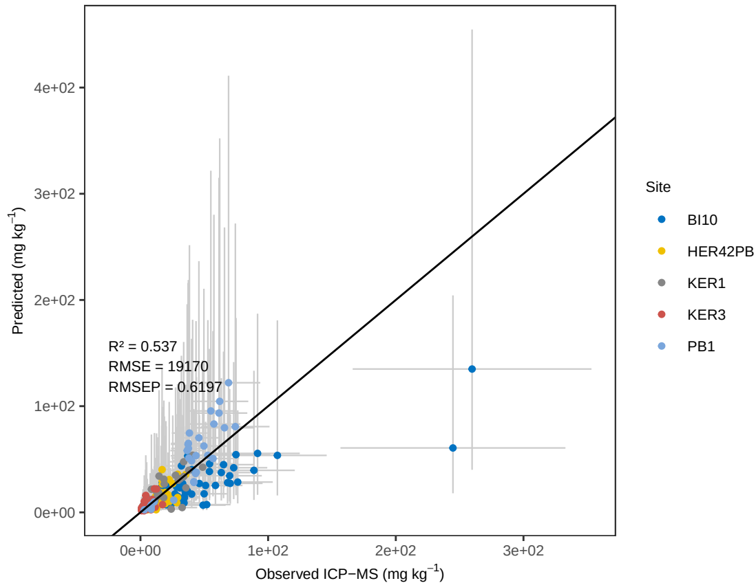
Fe OLS_weighted – ACE Predicted vs Observed (with errors)
