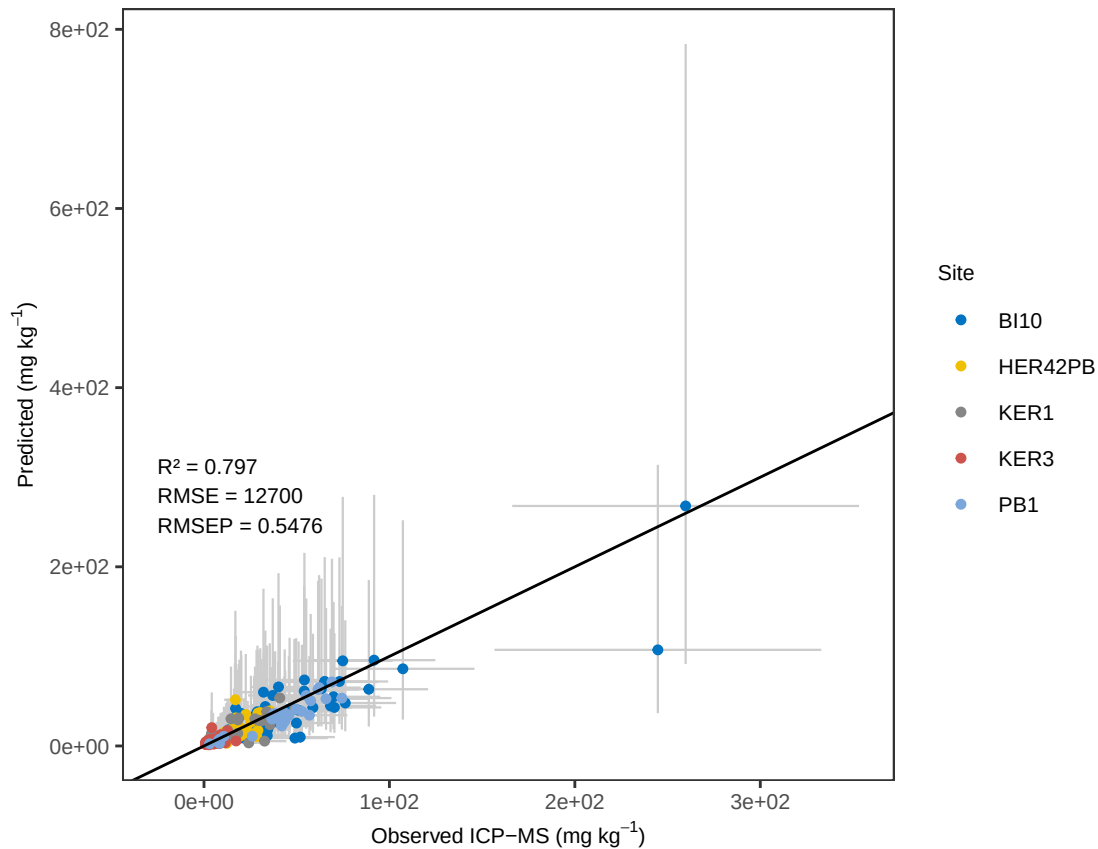
Fe PLS_LOO - ACE Predicted vs Observed (with errors)
