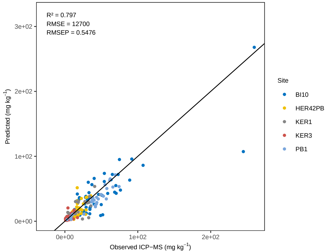
Fe PLS_kfold – ACE Predicted vs Observed
