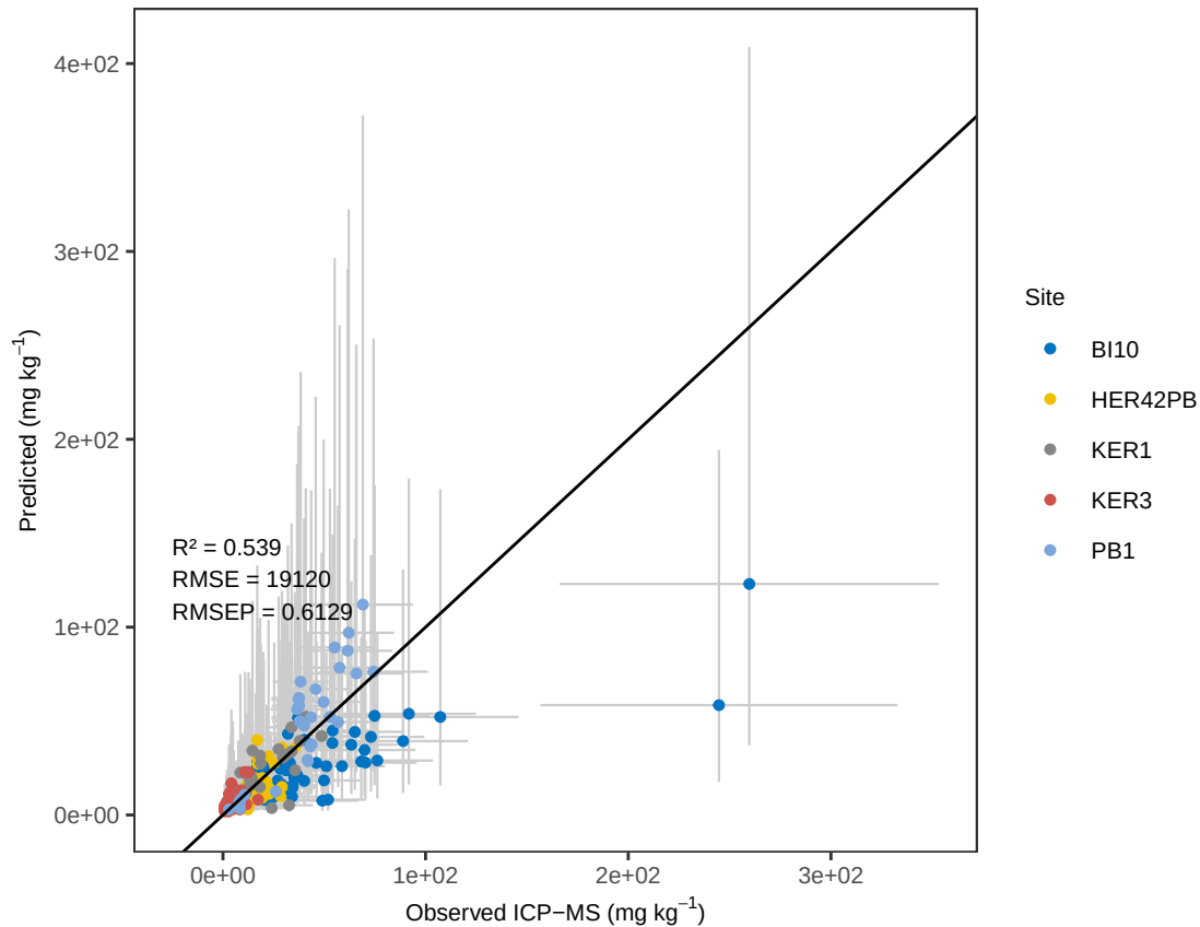
Fe WLS_weighted – ACE Predicted vs Observed (with errors)
