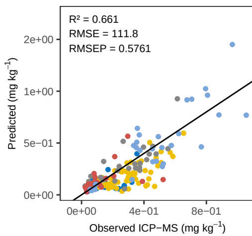
Mn WLS – ACE Predicted vs Observed
