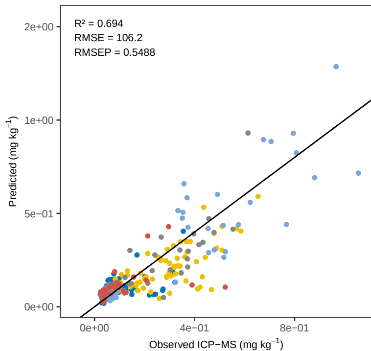
Mn Bayes – ACE Predicted vs Observed
