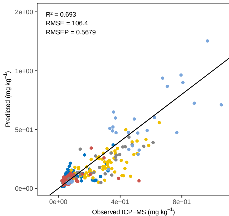
Mn PLS_kfold – ACE Predicted vs Observed
