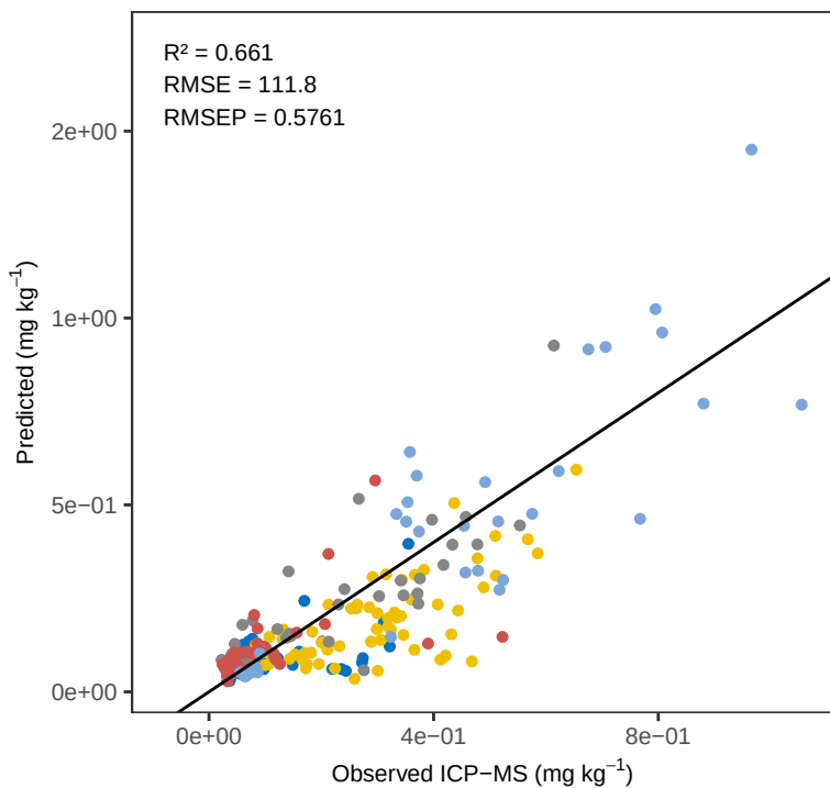
Mn OLS – ACE Predicted vs Observed
