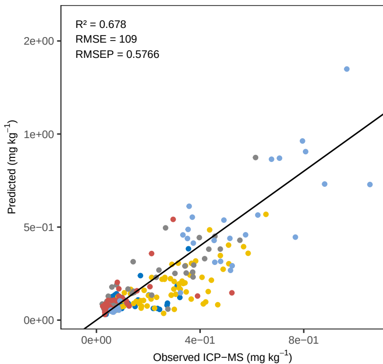
Mn WLS – ACE Predicted vs Observed
