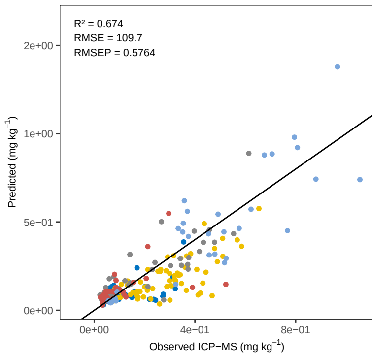
Mn WLS_weighted – ACE Predicted vs Observed
