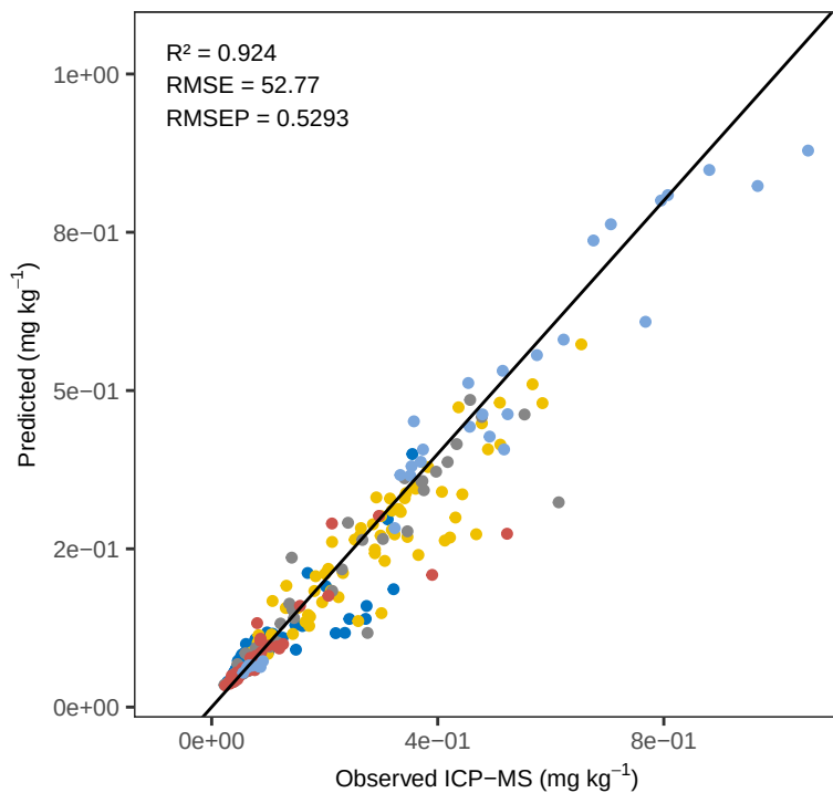
Mn RF – ACE Predicted vs Observed
