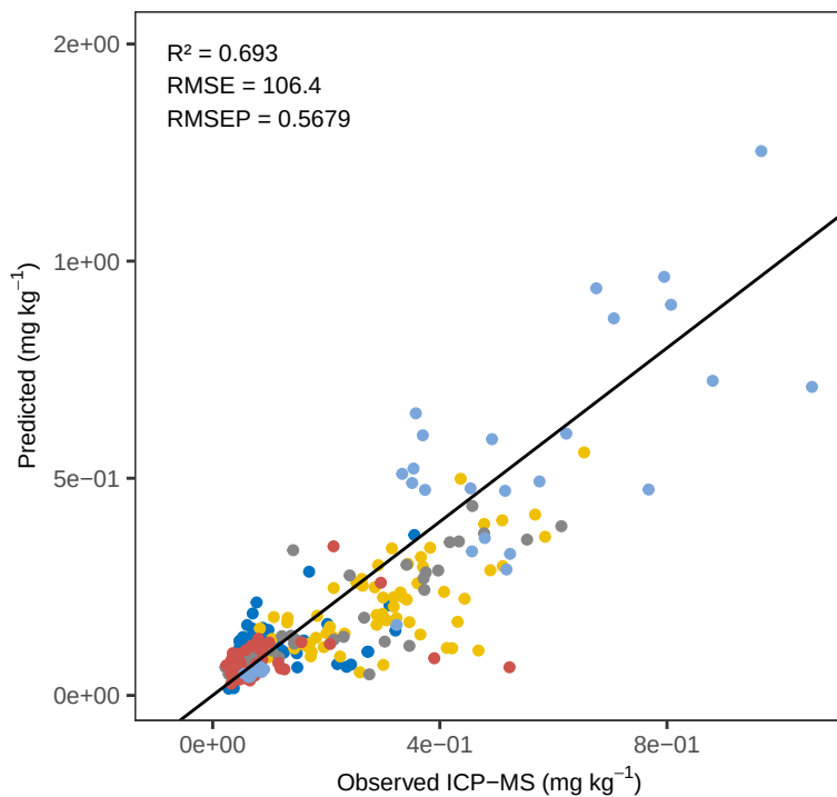
Mn PLS_LOO – ACE Predicted vs Observed
