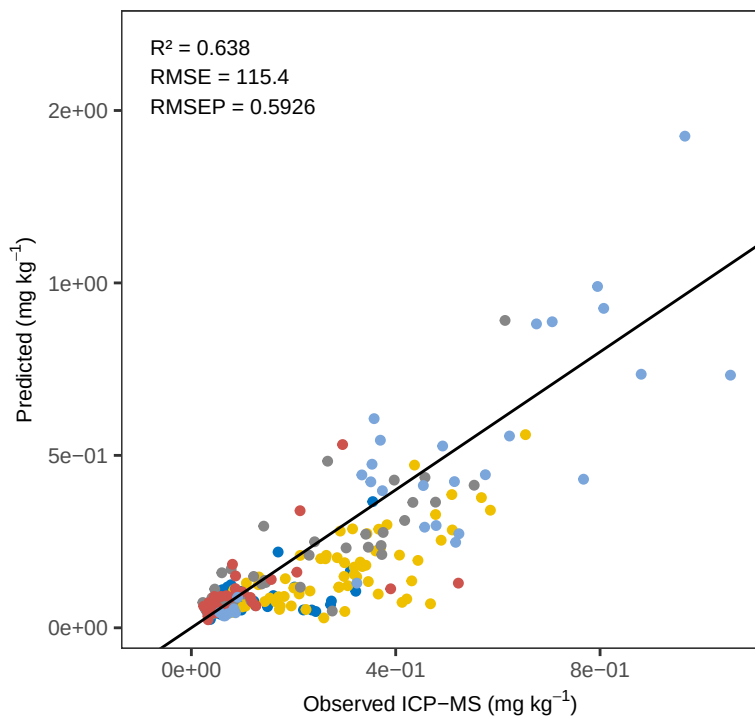
Mn OLS_weighted – ACE Predicted vs Observed
