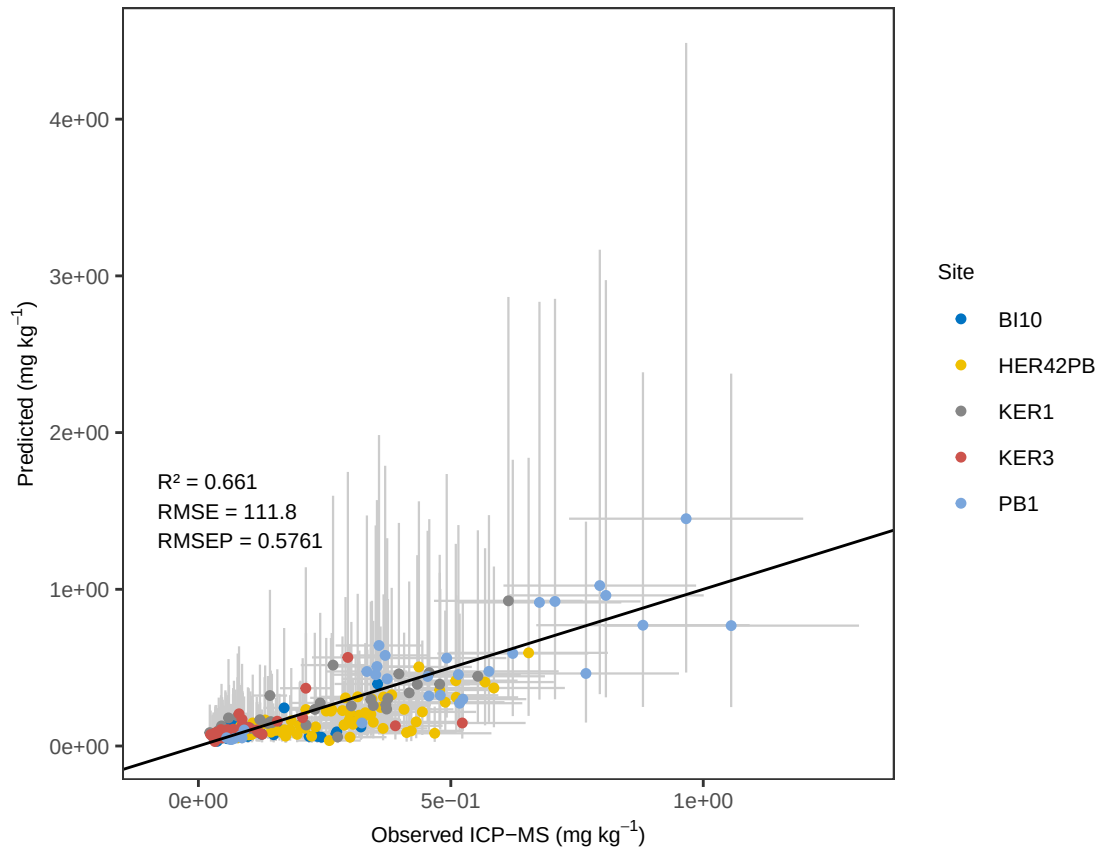
Mn OLS – ACE Predicted vs Observed (with errors)
