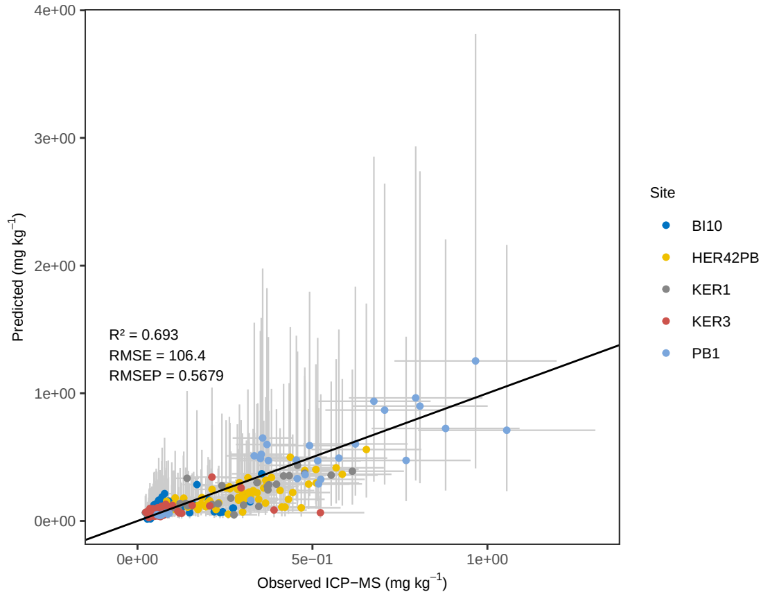
Mn PLS_LOO – ACE Predicted vs Observed (with errors)
