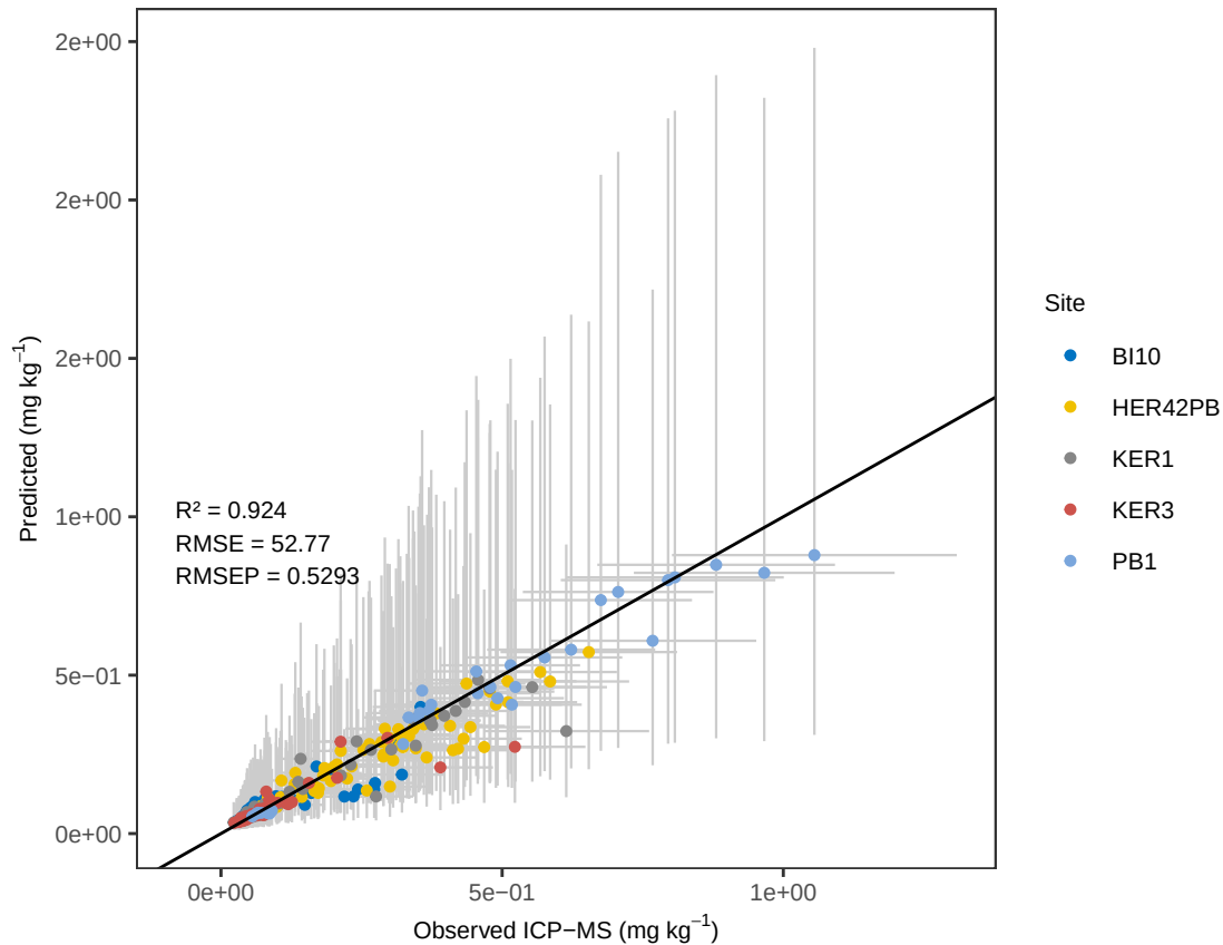
Mn RF – ACE Predicted vs Observed (with errors)
