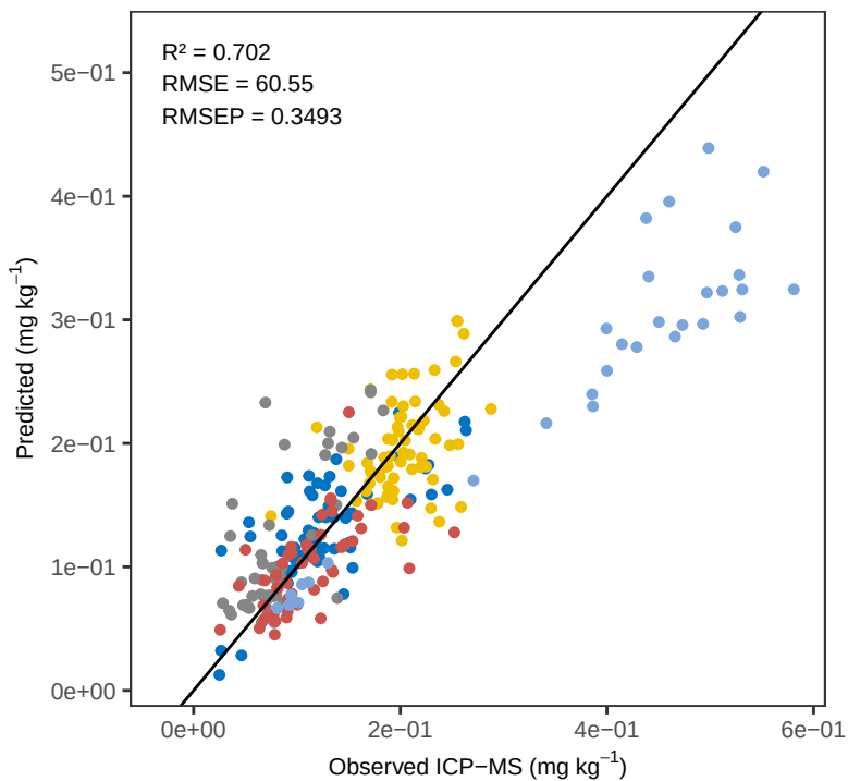
Sr PLS_kfold – ACE Predicted vs Observed
