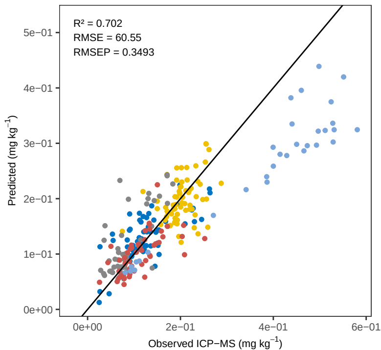
Sr PLS_LOO – ACE Predicted vs Observed
