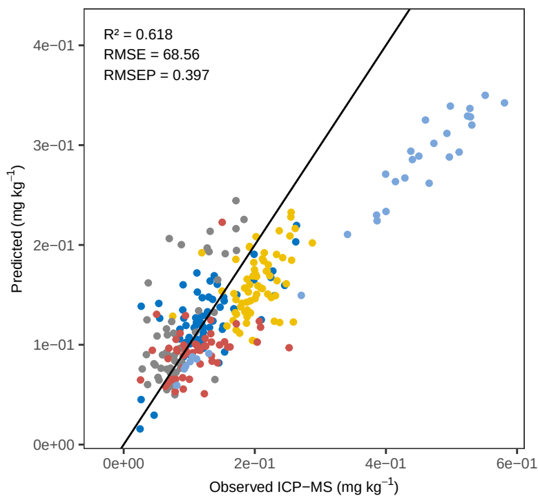
Sr OLS_weighted – ACE Predicted vs Observed
