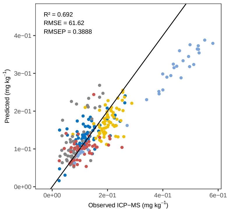
Sr WLS_weighted – ACE Predicted vs Observed
