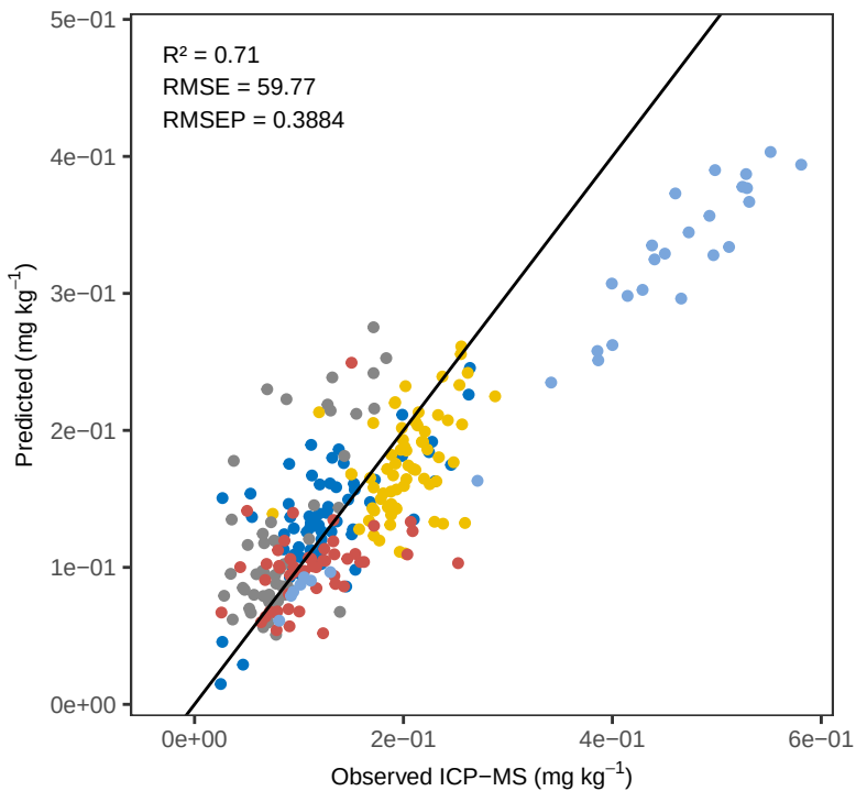
Sr OLS – ACE Predicted vs Observed
