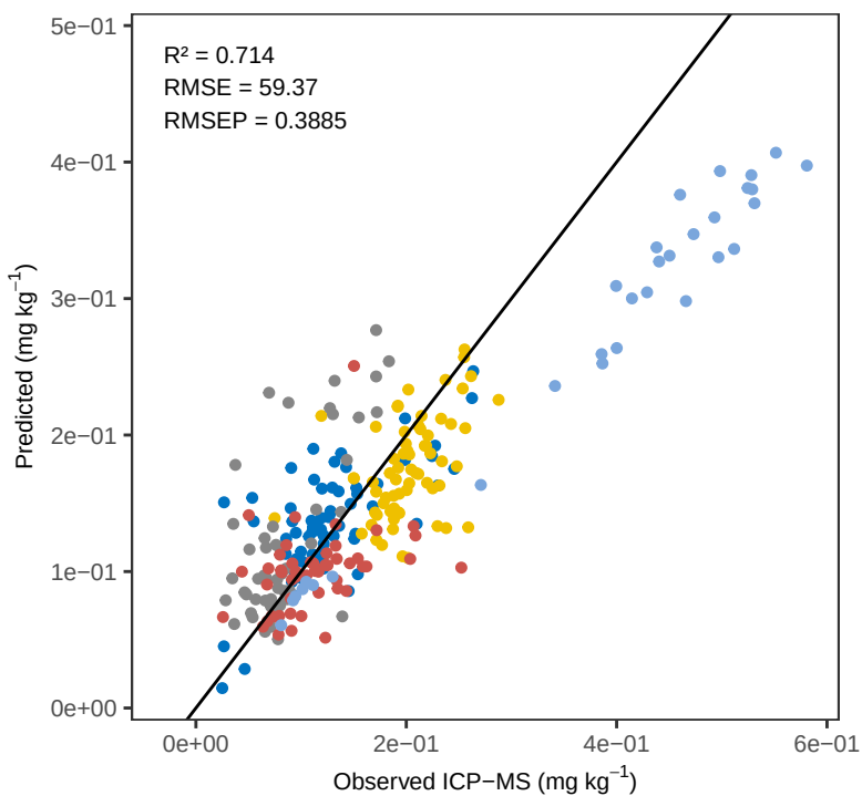
Sr WLS – ACE Predicted vs Observed
