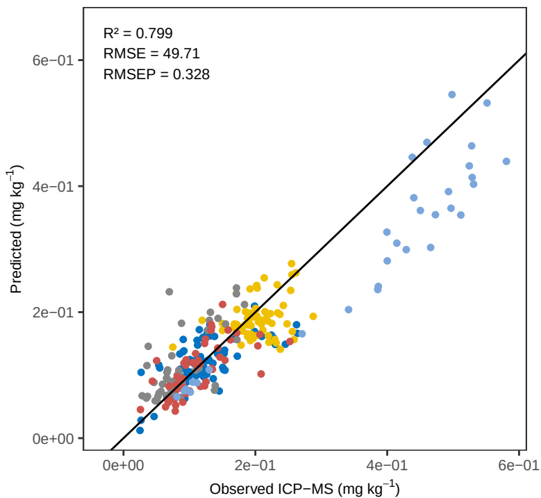
Sr Bayes – ACE Predicted vs Observed
