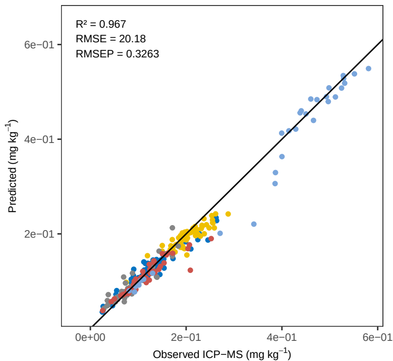
Sr RF – ACE Predicted vs Observed
