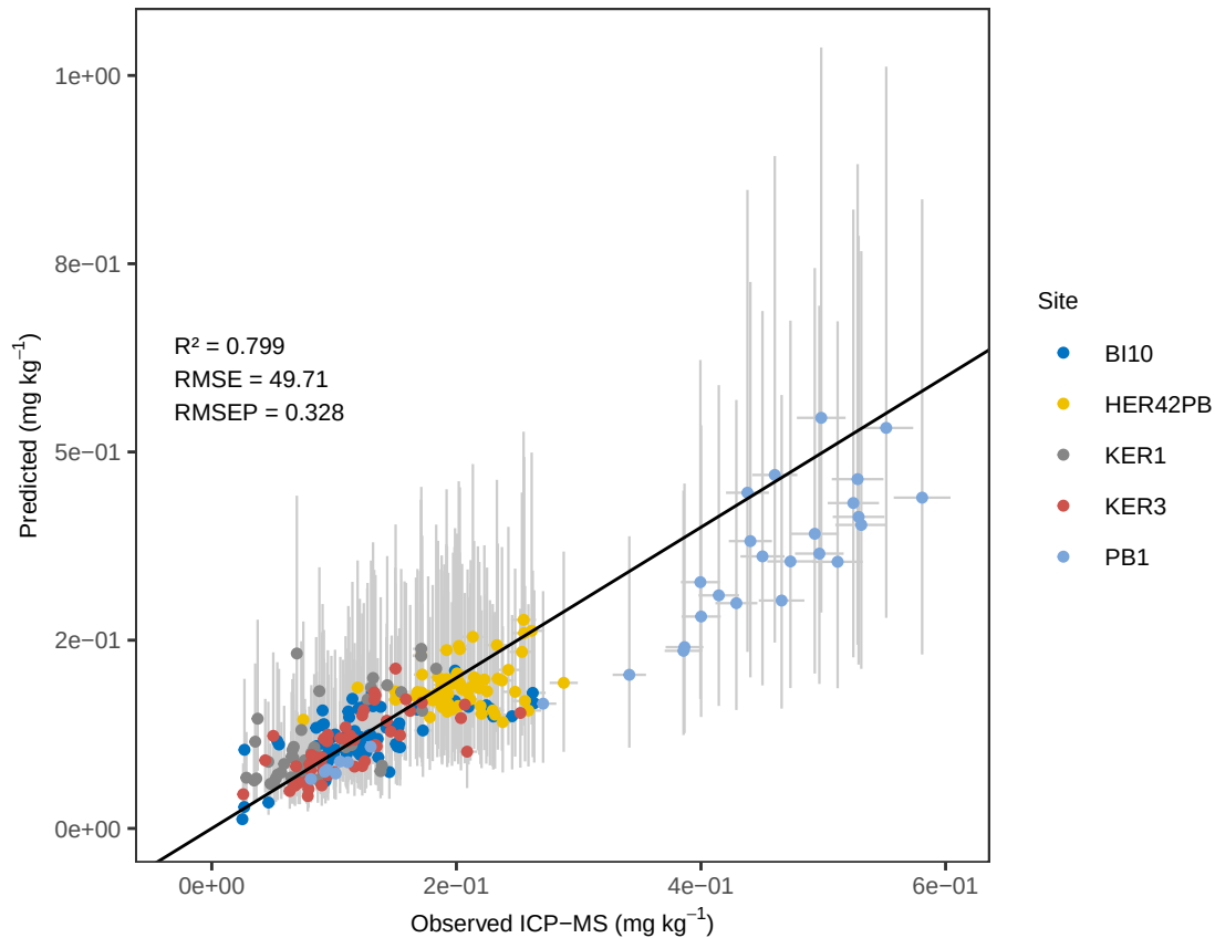
Sr Bayes – ACE Predicted vs Observed (with errors)
