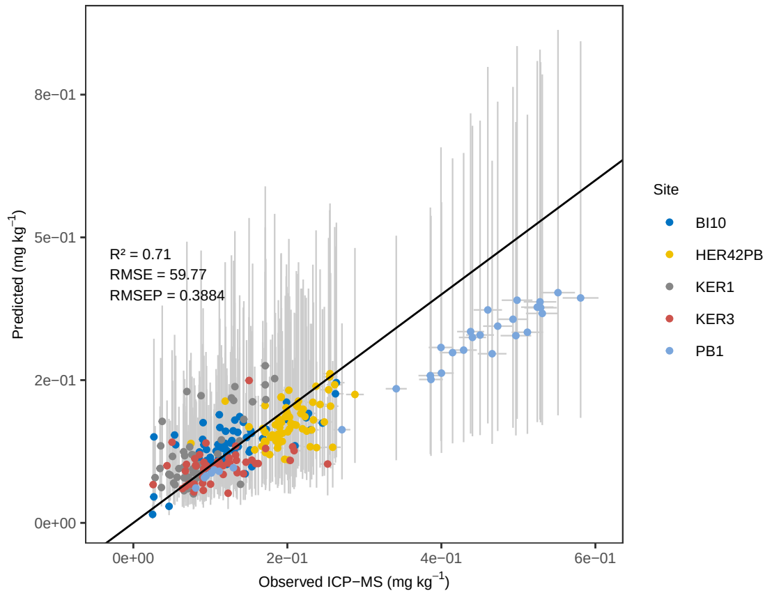
Sr OLS – ACE Predicted vs Observed (with errors)
