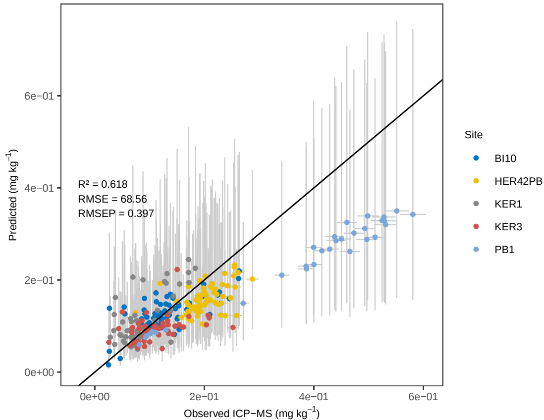
Sr OLS_weighted – ACE Predicted vs Observed (with errors)
